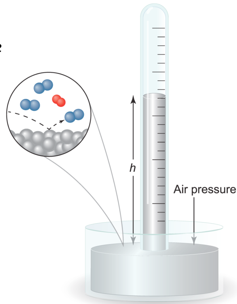
Figure 7.3 Simple Barometer
